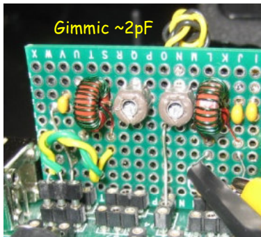
Component 10MHz BPF
