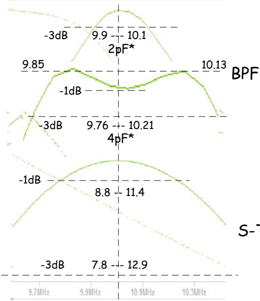
Component 10MHz BPF
