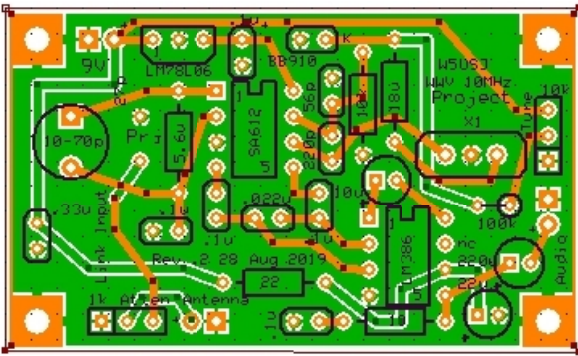
Express PCB WWV + Circuit Board
